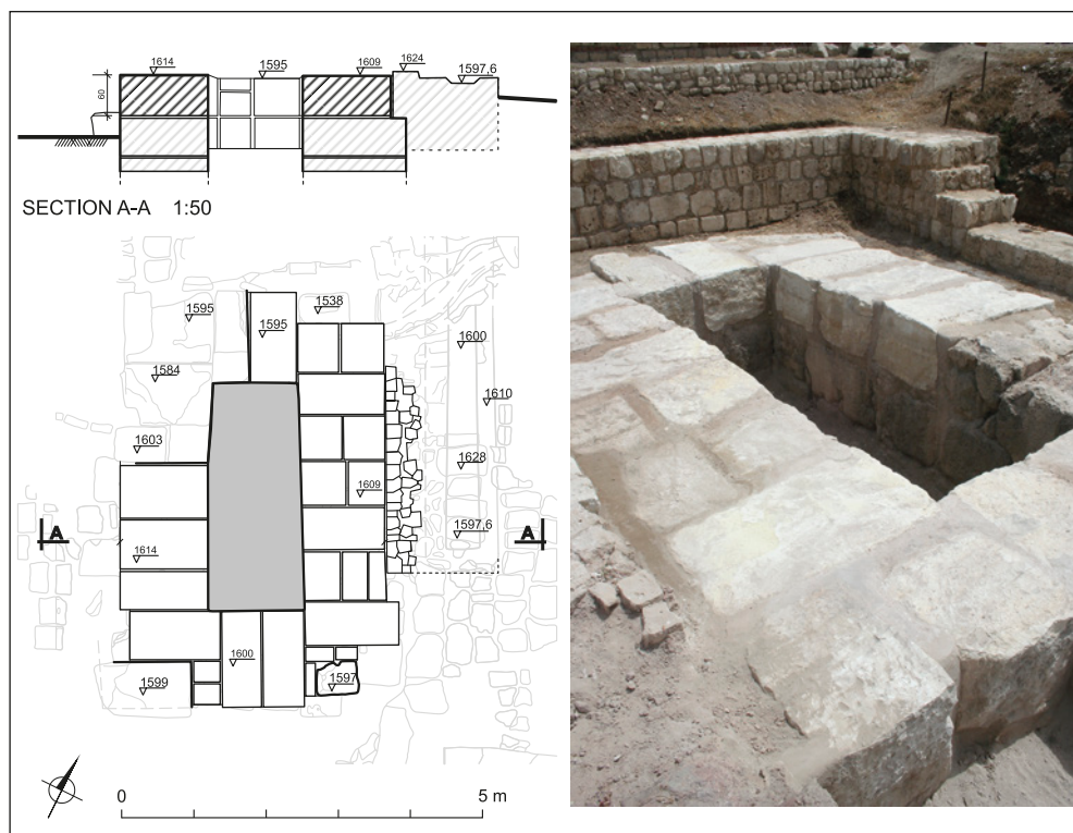
Fig. 21. Southwestern well in the cistern: left, plan; right, view after restoration (Drawing and photo A. Piszczewski)
