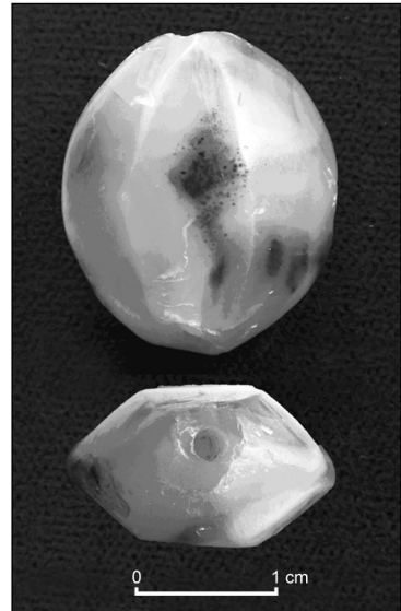
Fig. 3. Almond-shaped bead made of carnelian, Troy (After Blegen et alii 1953: Cat. No. 35-531, Fig. 298; photo M. Pieniżek)
