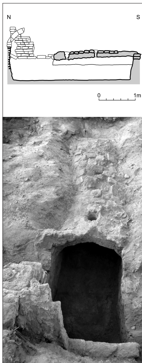
Fig. 4. Cellar in room K.3–K.4, view of the entrance shaft and vaulted roof seen from the north (left) and section looking east (Photo W. Godlewski, drawing E. Krupski, PCMA archives)
