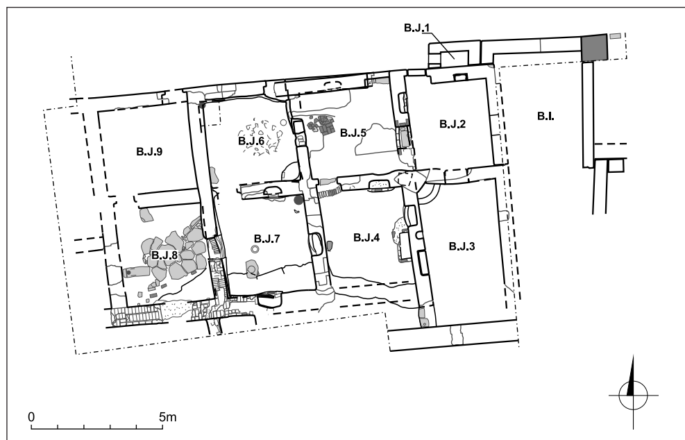
Fig. 8. Plan of Building J, state after the 2008–2009 seasons (Plan S. Maślak, PCMA archives)
