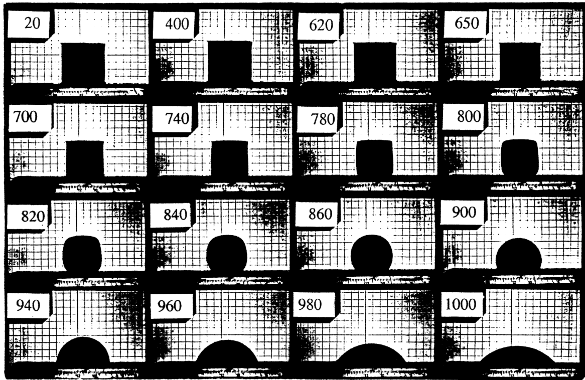
Fig. 1. Sample No. 3 during heating, observed under a high-temperature microscope.
